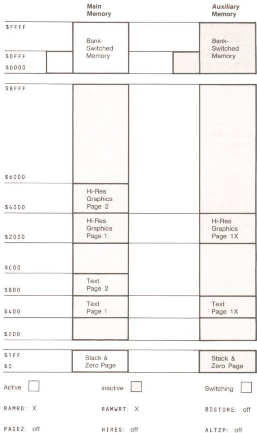
Figure 3-2. Effect of Switching RAMRD and RAMWRT with 80STORE Off
